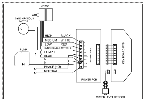
WINTER 80XLi, HI COOL i
