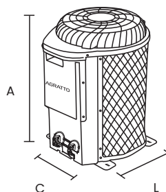
9K Btus - EXT. (CxLxA) 478X390X550mm
