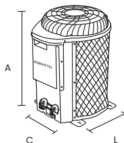
24K Btus - EXT. (CxLxA) 480X550X680mm
